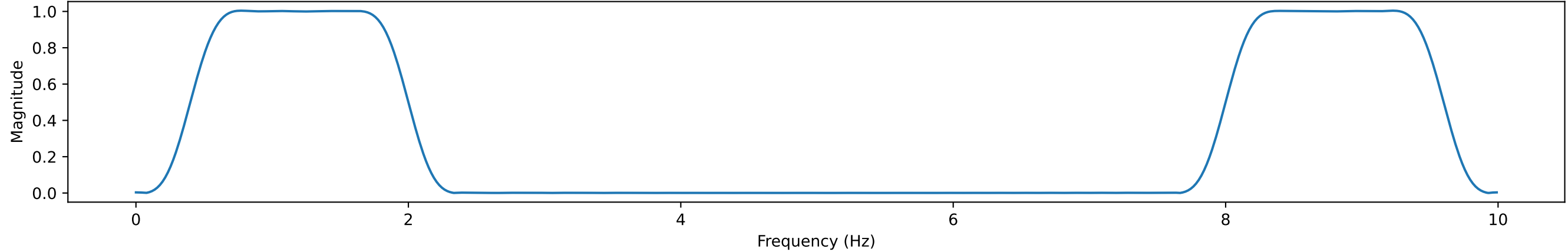
Frequency Response of Filter h3[n]
