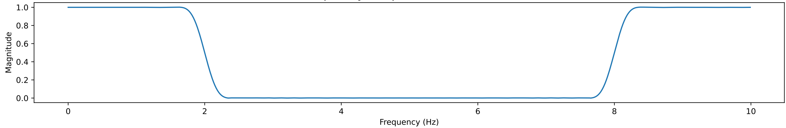
Frequency Response of Filter h2[n]
